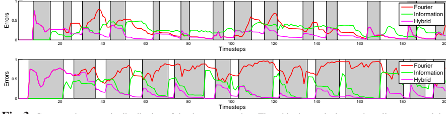
Fig. 3. Compare the errors in distribution of the three approaches. The white intervals denote the rollup steps and the grey intervals denote the conditioning steps.
