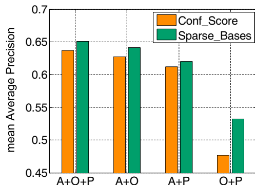
Figure 3. Comparison of the methods by removing the confidence scores obtained from attributes (A), objects (O), and poselets (P) from the feature vector, one at a time. The performance are evaluated using mean Average Precision on the PASCAL dataset.
