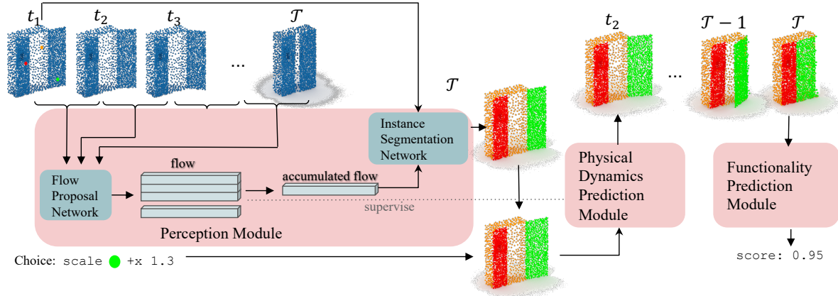
Figure 3. Our proposed FixNet. The point cloud videos are first fed into the flow proposal network which outputs the flows of the points. The flows, and the point cloud of the malfunctional object (which is also the first frame of the video) are input to the segmentation network to produce part instances. Given a choice represented as domain-specific language (DSL), the part referred to in the choice is retrieved via the root point, and modified according to the DSL. The point cloud of the fixed object is then fed into the physical dynamics prediction module, together with the part instances, to predict the future states of the object. The physical dynamics module is trained on the pseudo labels provided by the flows. The last state is input to a functionality prediction module which outputs a functionality score.
