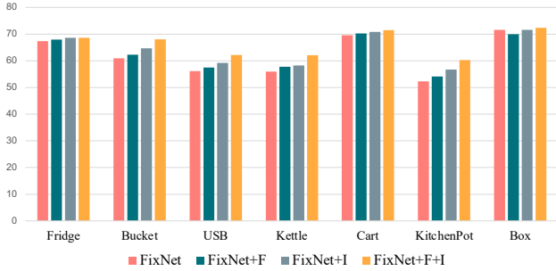
Figure 6. Model Diagnosis. Y-axis represents test accuracy. Adding ground-truth perception can boost the accuracy of FixNet to some extent, especially for categories with low accuracies.
