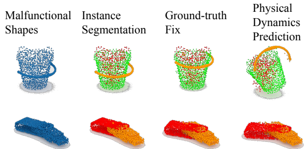
Figure 5. Failure cases by FixNet. For the bucket, the instance segmentation network cannot segment water from the bucket, and the dynamics prediction module disjoins the parts. For the USB, the overlapping of parts result in inaccurate physical simulation. For example, the shell of the USB in Figure 5 is embedded in its body, making the segmentation extremely hard. Since the hierarchical modeling in DPI-Net forces the particles in an instance to have similar dynamics, one part can be blocked by another static part due to intermediate overlapping particles. Therefore, the USB shell that is embedded in the body fails to rotate, while some USBs with separating shell and body manage to function well. In another case, we show the bucket full of water. It’s hard to tell the water apart from the bucket body. We find that a large amount of the water particles are segmented into the body part. Since DPI-Net tends to unify the transformations within an instance, the bucket body might be dragged by the water when it spreads out, making the functionality prediction incorrect. As we can see, the fixed bucket should be lifted vertically, but it leans away. The second weakness is that the physical dynamics predictor fails to simulate articulated parts very well. For example, the handle of the bucket is disjointed. This also happens to the cart wheel in the qualitative examples. How to adjust dynamics model for articulated objects and objects with multiple parts is worth delving into.
