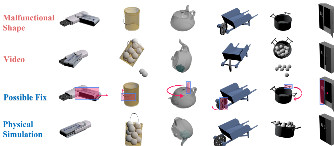
Figure 1. We introduce FIXIT, a dataset that requires machines to fix malfunctional objects based on functionality. Each malfunctional object is paired with a video presenting how the object is interacted. Functionality of fixed objects can be evaluated via physical simulation.
