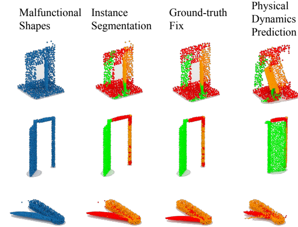
Figure 7. Examples of generalization. For the first door, both segmentation and simulation are incorrect. For the second the door, the segmentation is incorrect but the simulation is right. For the USB, the segmentation is wrong and the simulation is half-right. For the second door, although the segmentation is also incorrect, the physical dynamics predictor manages to simulate the perfect results. For the USB, the model simulates the first half of the trajectory accurately, but then stops. This might be due to the slightly different interaction ways of USBs and knives.
