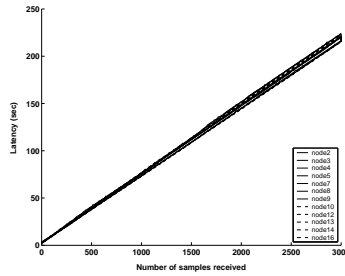
Fig. 10. Latencies measured in the seismic- test structure deployment
