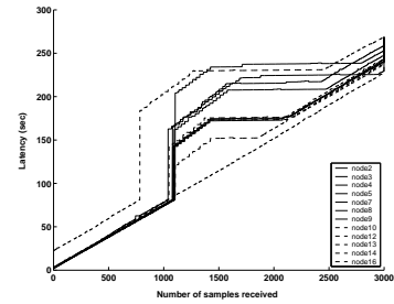
Fig. 11. Latencies measured when one Star-Gate was unplugged during the experiment
