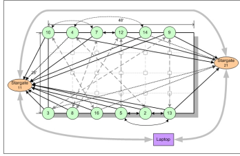
Fig. 9. Layout of the motes in the seismic structure
