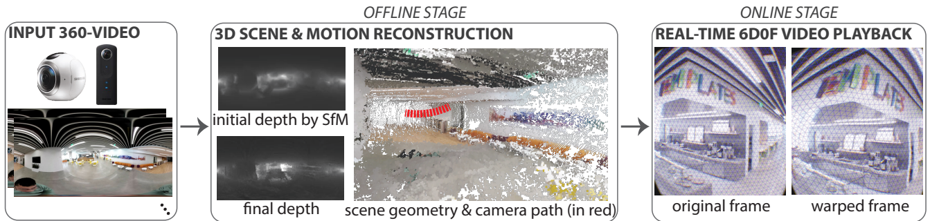
Figure 1: Given a 360-video captured by a single spherical panorama camera, in an offline pre-processing stage, we recover the camera motion and the scene geometry first by performing structure-from-motion (SfM) followed by dense reconstruction. Then, in real-time we playback the video in a VR headset where we track the 6-DOF motion of the headset and synthesize new views by a novel warping algorithm.
