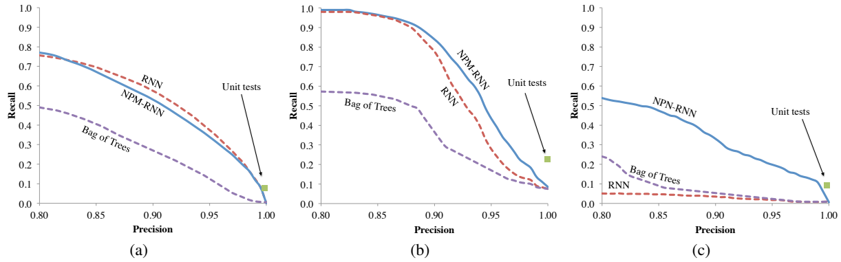
Figure 3. Recall of feedback propagation as a function of precision for three programming problems: (a) \Omega_1 , (b) \Omega_2 , and (c) \Omega_3 . On each, we compare our NPM-RNN against the RNN method and two other baselines (bag of trees and unit tests).
