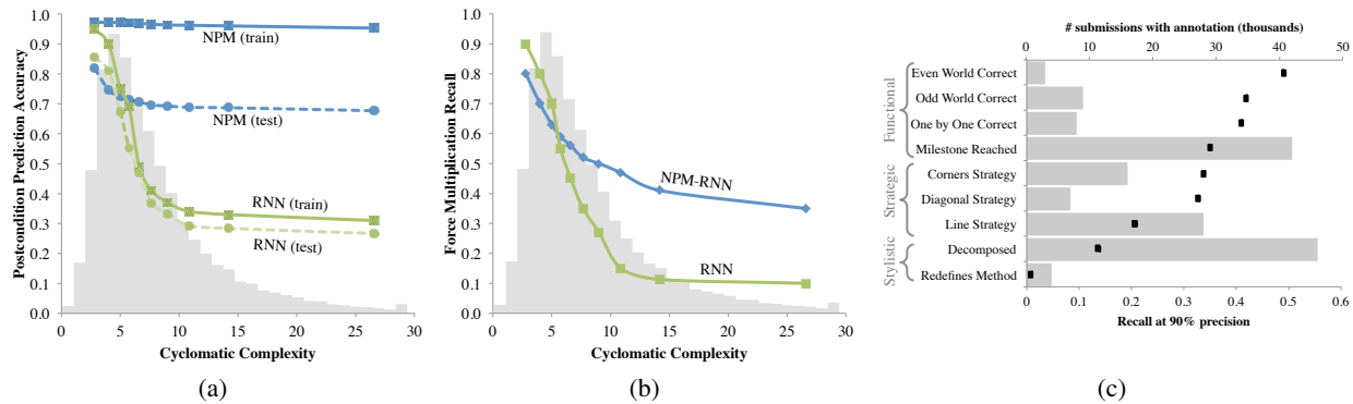
Figure 4. (a) NPM and RNN postcondition prediction accuracy as a function of cyclomatic complexity of submitted programs; (b) NPM-RNN and RNN feedback propagation recall (at 90% precision). Note that the ratio of human graded assignments to number of programs is much higher in this experiment than Figure 3; (c) A breakdown of the accuracy of the nonparametric model by feedback type for \Omega_3 (black dots). The gray bars histogram the feedback types by frequency.
