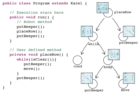
Figure 1. We learn matrices which capture functionality. Left: a student partial solution. Right: learned matrices for the syntax trees rooted at each node of placeRow .
