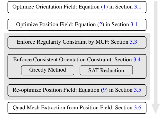
Figure 2: The pipeline of QuadriFlow. The white nodes are from Instant Meshes [JTSPH15]; the shaded nodes are our contribution.
