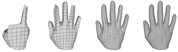
131 vertices 344 vertices 1486 vertices 3365 vertices Figure 14: A limitation of our method for coarse mesh generation. As we approximate an MIP problem as a minimum cost flow problem, geometric details can be lost when the target mesh density is low.
