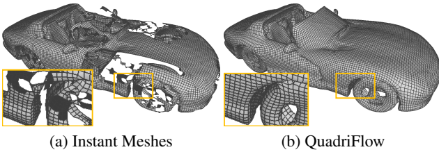
(a) Instant Meshes (b) QuadriFlow
