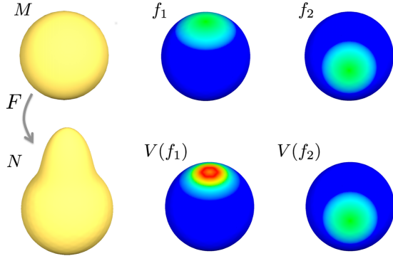
Figure 2: Given a pair of shapes M and N (left column) and a functional map F , the shape difference V is a linear operator, which for every function f on M produces another function V(f) on N which intuitively encodes how much f is distorted by F (center and right). Note that f_1 is supported in an area that deforms under the map, and f_2 in an area that does not.
