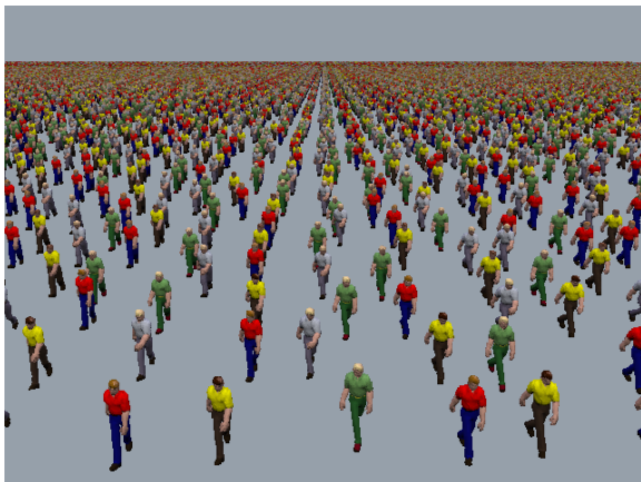
replicated poser models, 90000 objects, 575 million triangles, rendering time 294 msec (splat size 2 \times 2 )
