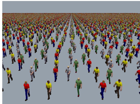
(d) replicated poser models, 90000 objects, 575 million triangles, rendering time 294 msec (splat size 2×2)
