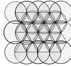
Figure 6: The worst-case sample distribution is a tightest packing of circles.
