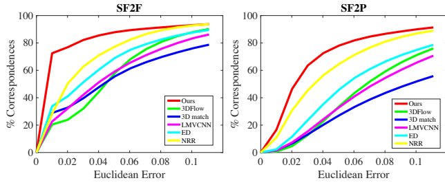
Fig. 7. Percent of correspondences which have Euclidean error smaller than a threshold. The x-axis corresponds to different thresholds.
