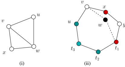
Fig. 15. (i) Node v is not stuck in the direction of \angle uvx after the node w fails. (ii) There was a hole bounded by vwt_1t_2t_3uv . After the failure of node w , the hole is bounded by vxyt_1t_2t_3uv .
